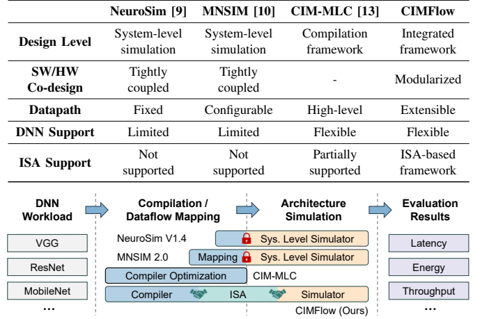
Fig. 1. Comparing CIMFlow with recent design and evaluation frameworks for CIM architectures.
